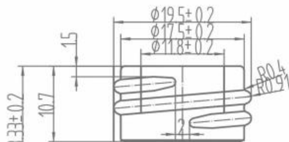
20-410 Neck
